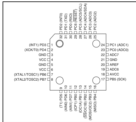
Figure 5. ATmega8 TQFP
