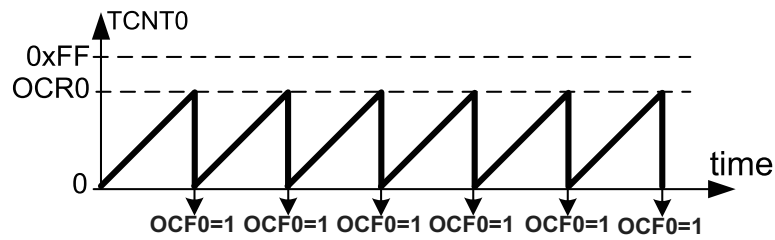
Figure 10. Timer/Counter 0 CTC Mode
