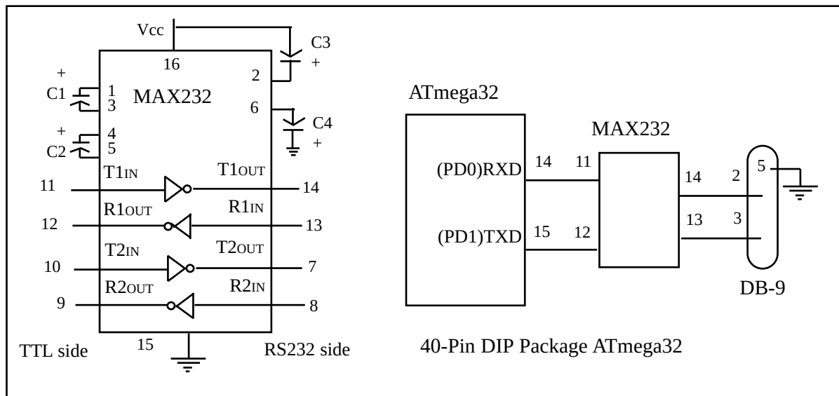
Figure 8. (a) Inside MAX232 and (b) Its Connection to the ATmega32 (Null Modem)
