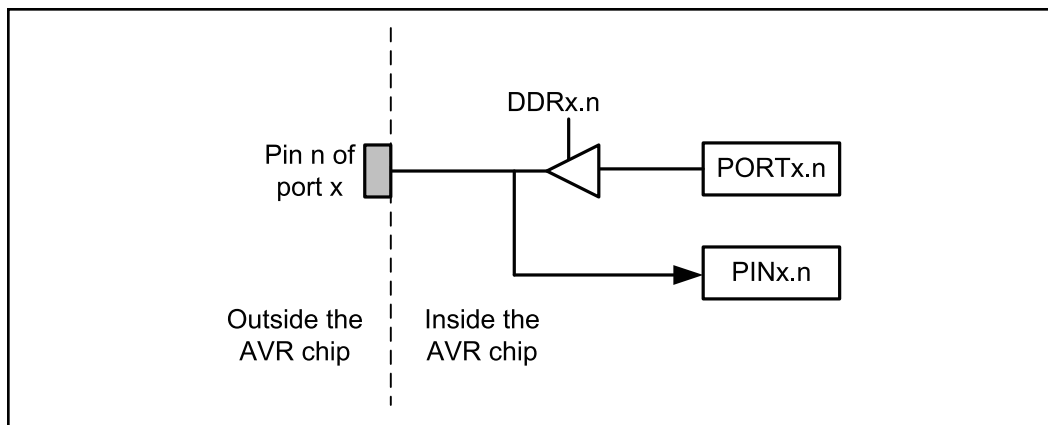
Figure 3. The I/O Port in AVR
