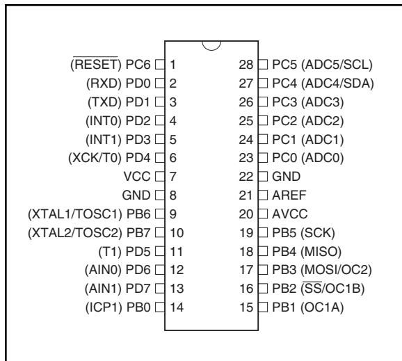
Figure 4. ATmega8 DIP
