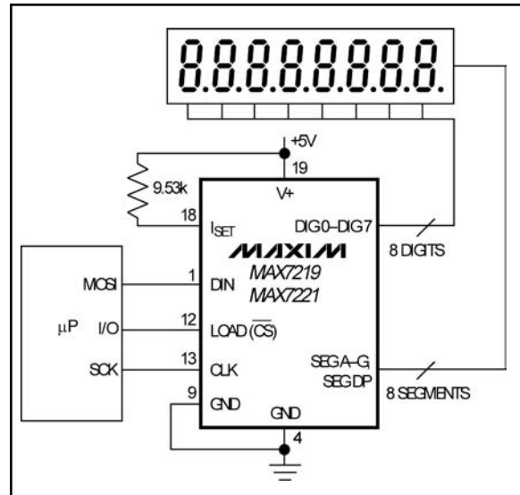
Figure 7. MAX7221 Connections
