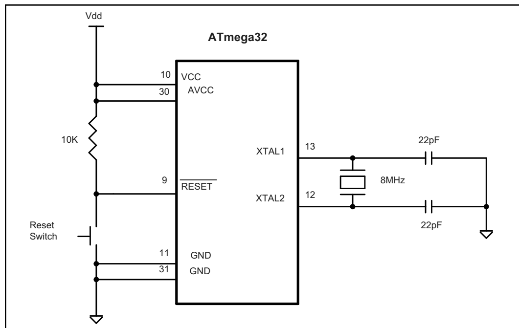
Figure 2. Minimum Connection for ATmega32
